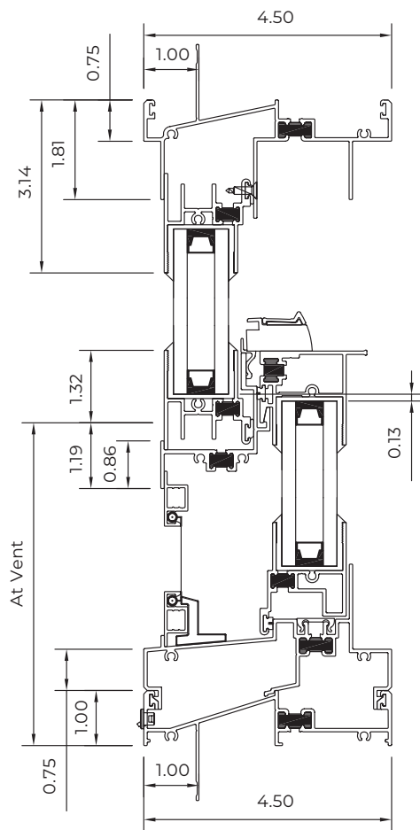
Vertical Section Single Hung 1.00" Nail-Fin Frame
