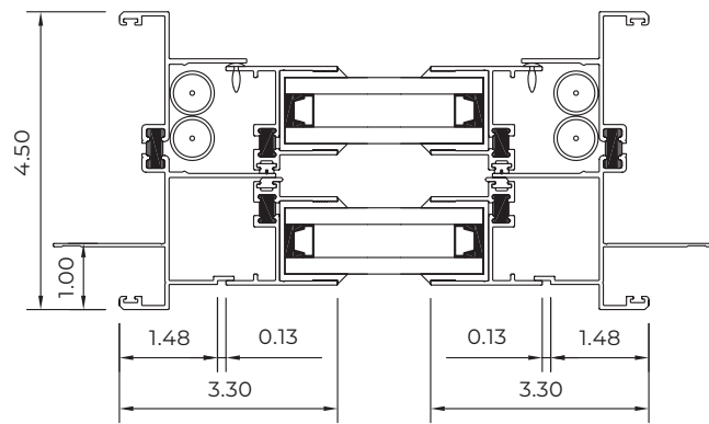
Horizontal Section Single Hung 1.00" Nail-Fin Frame
