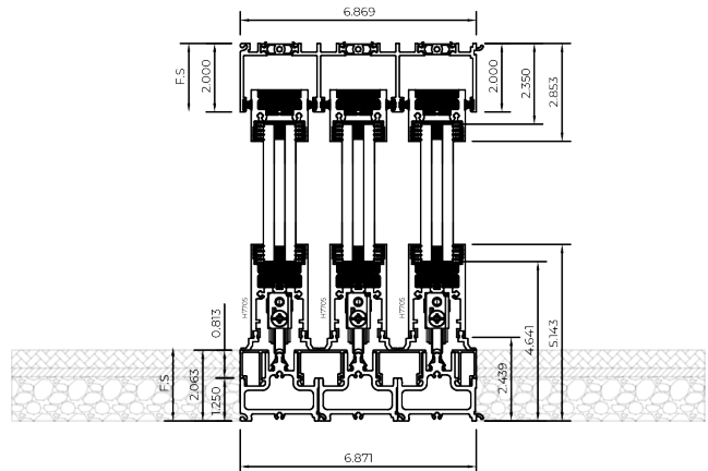
Flush Water Management Threshold
