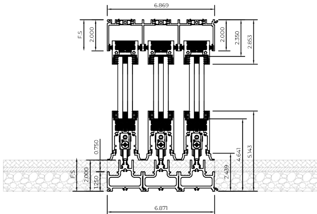
Thinline Water Management Threshold
