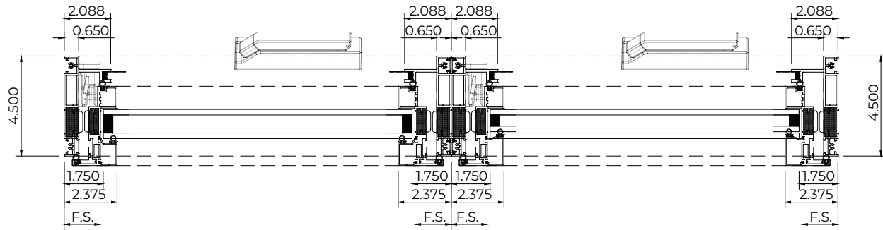
Casement - Mull Unit
