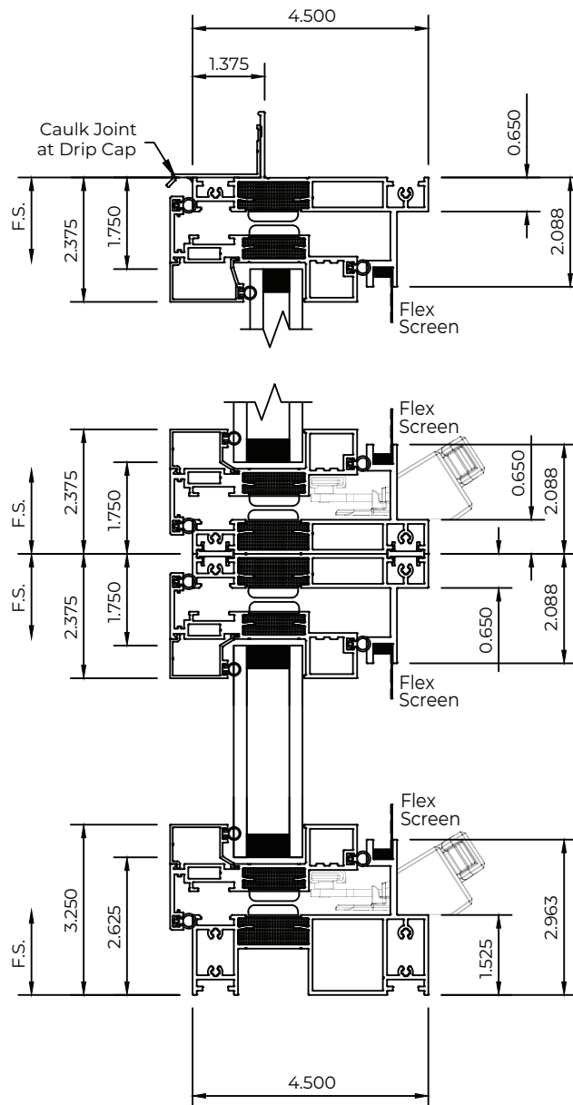
Casement Over Fixed - Mull Unit
