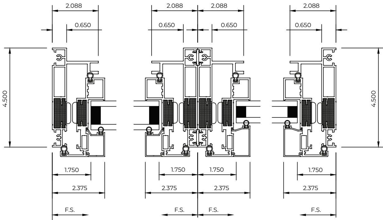
Fixed Sash - Muller Unit
