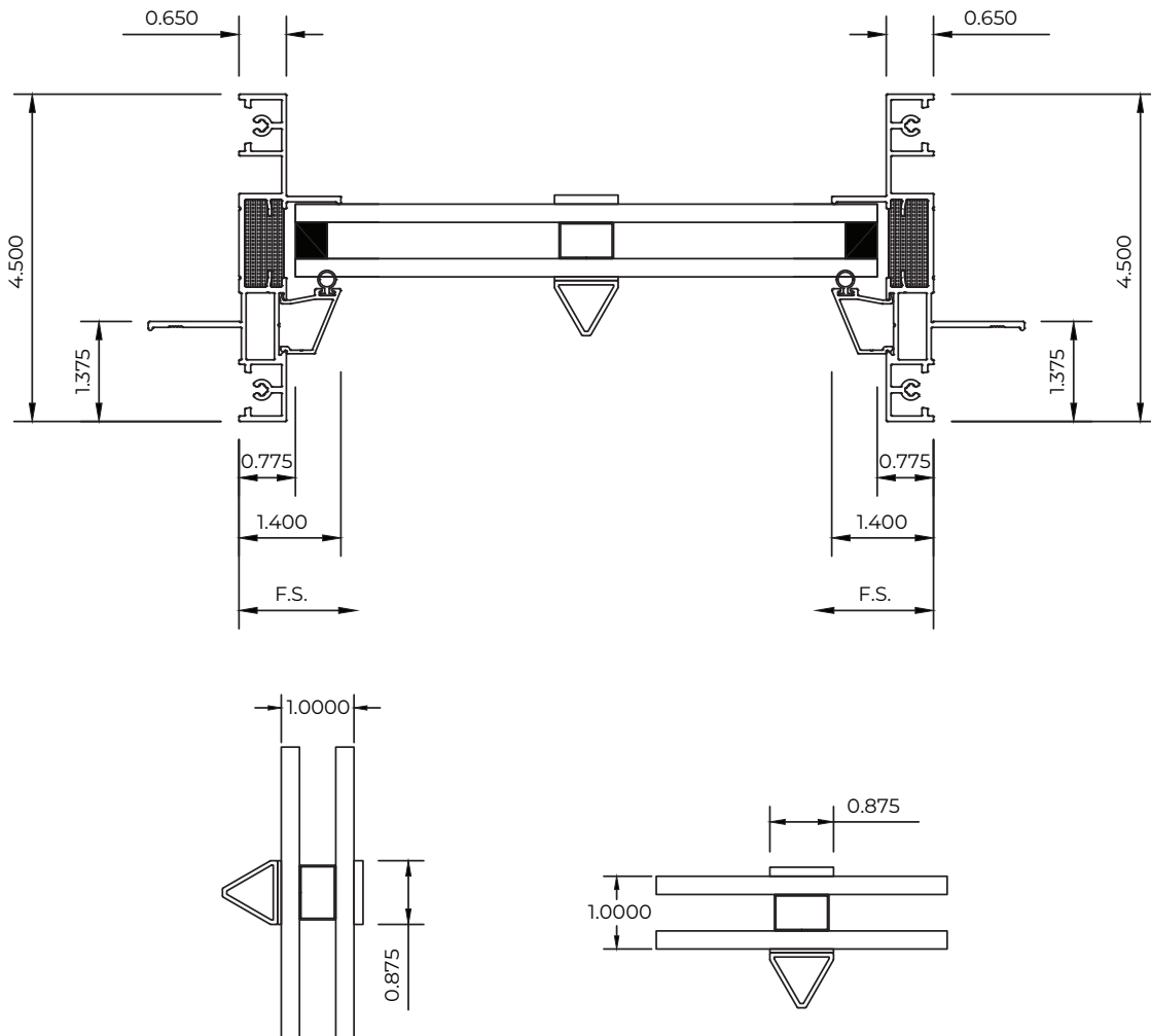
Beveled Grids
