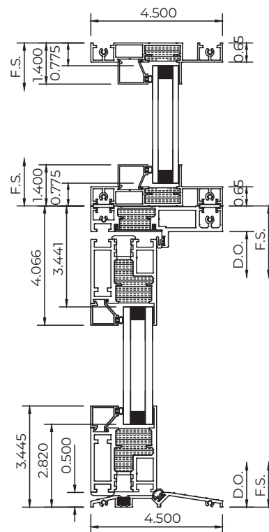
Equal Leg Frame Low-Profile Threshold
