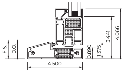
Standard Threshold
