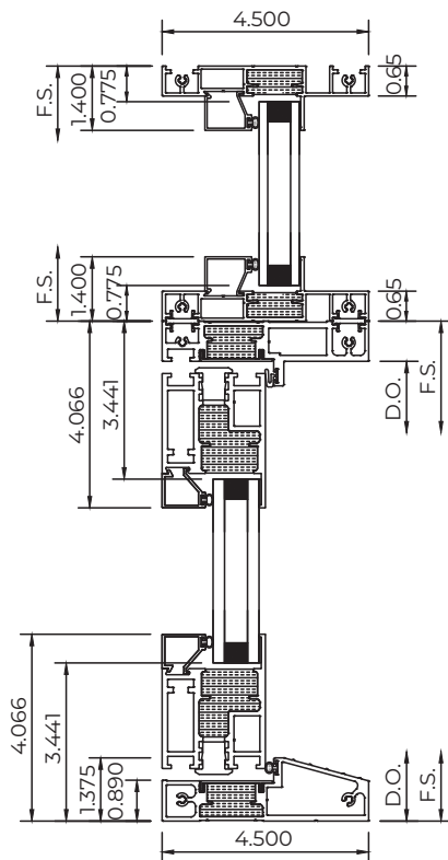
Equal Leg Frame Standard Threshold
