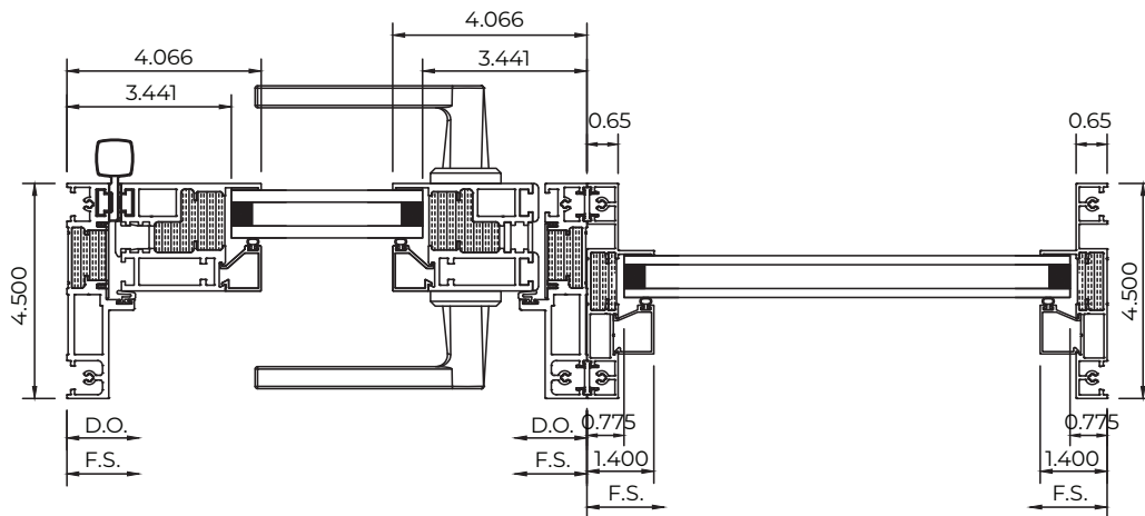
Equal Leg Frame
