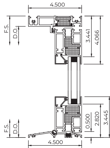
Equal Leg Frame Low-Profile Threshold
