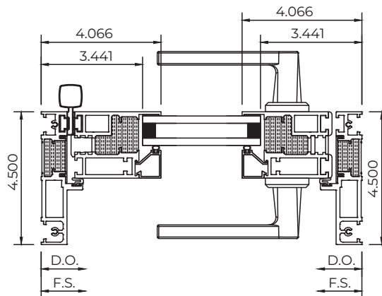
Equal Leg Frame
