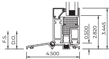
Commercial Threshold
