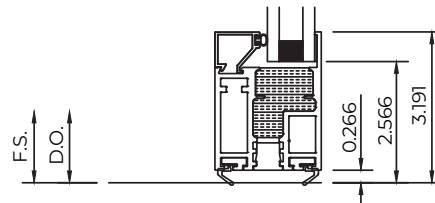
No Threshold
