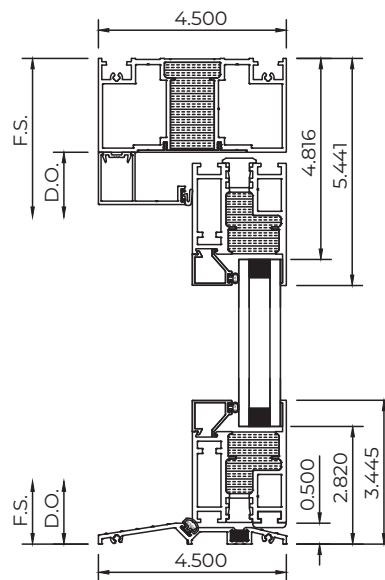
Equal Leg Frame Concealed Overhead Closure Head Low-Profile Threshold
