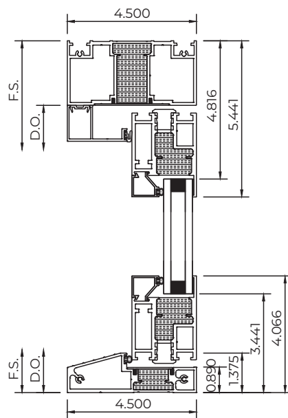
Equal Leg Frame Concealed Overhead Closure Head Standard Threshold
