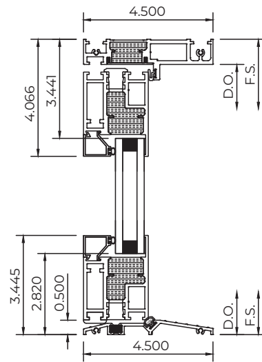
Equal Leg Frame Low-Profile Threshold
