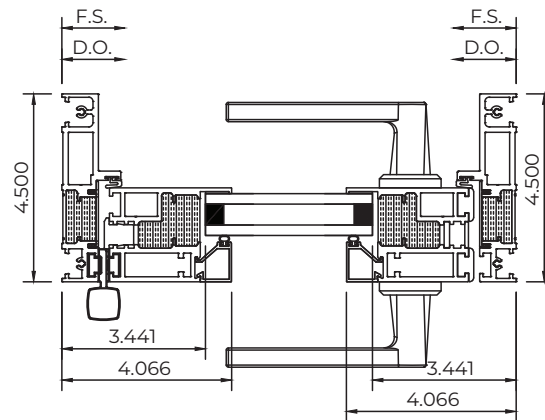
Equal Leg Frame
