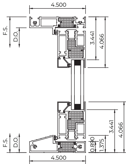
Equal Leg Frame Standard Threshold
