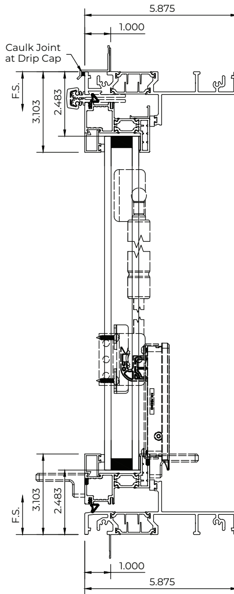
Nail Fin Drip Cap - 1.30 Glass With Sill
