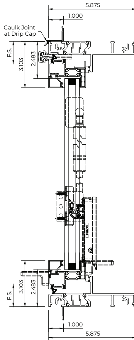
Nail Fin Drip Cap - 1.00 Glass With Sill
